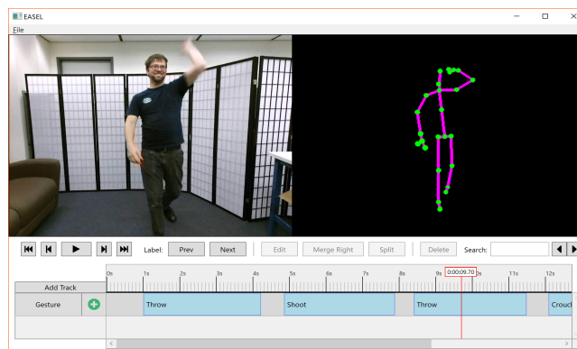
Figure 1. EASEL's user interface, showing the video player (top) and the annotation timeline (bottom).
